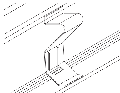
AXSPTHDC – Hold Down Clip
