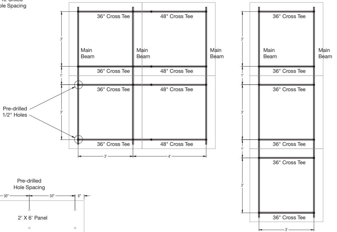
2' x 6' Panel Layout
