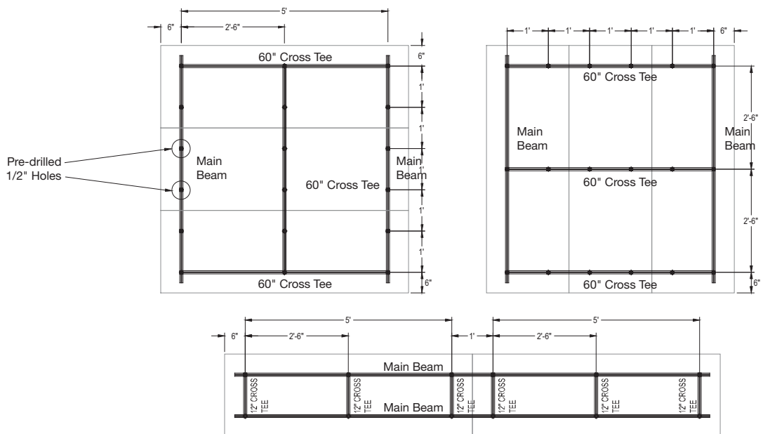
2' x 6' Panel Layout
